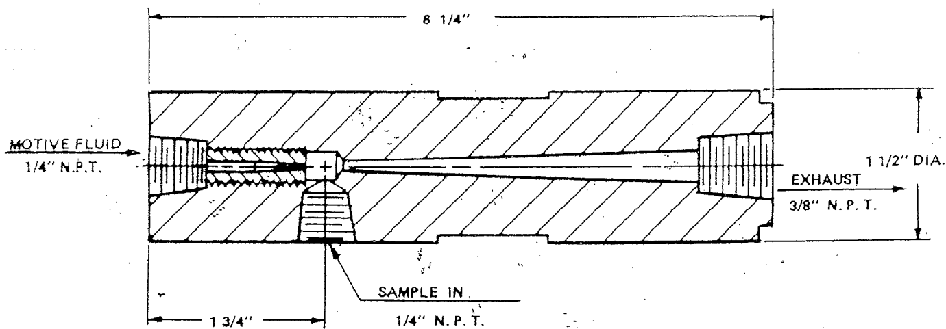
ASPIRATOR DETAILS
